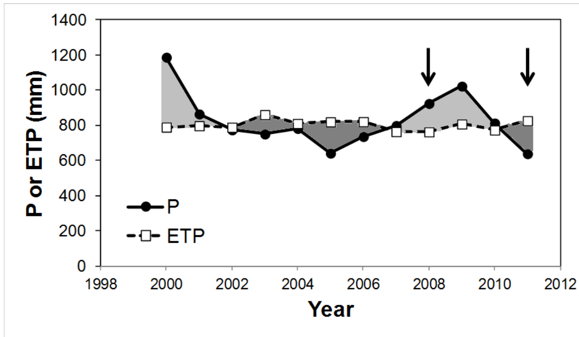
Figure 2 Annual micrometeorological conditions in Cestas (Cestas, 0°41'04.7" O, 44°44'27.2" N, weather station n°33122004, MétéoFrance, Agroclim database) for the last twelve years. P annual precipitation (mm), ETP potential evapotranspiration (mm) calculated with the Turc equations. Light gray areas corresponded to water surplus whereas dark gray areas corresponded to water deficit. Studied years are indicated by arrows.
