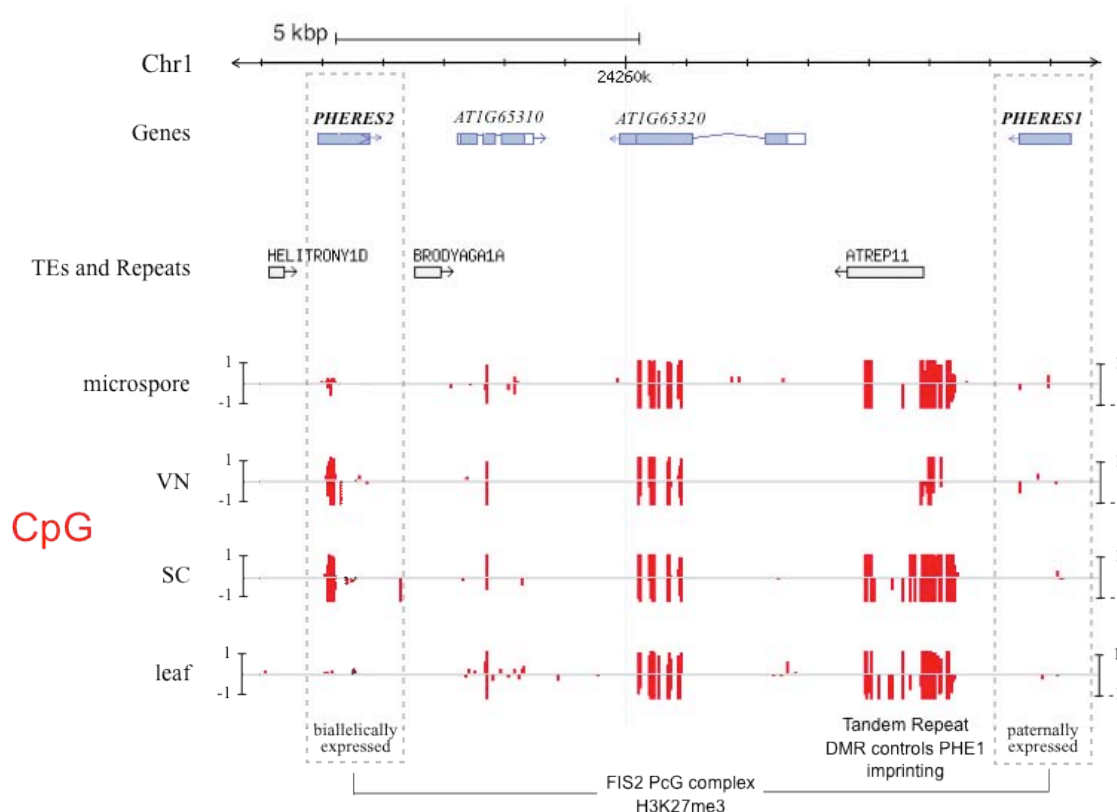
Figure 4.3 - DNA methylation at TEs neighboring paternally and maternally imprinted genes and CG methylation of PHERES genes. (A) Relative DNA methylation at TEs neighboring imprinted genes. CHG and CHH methylation in pollen and sporophytic tissues is much lower in paternally expressed genes (PEGs) than that of maternally expressed genes (MEGs). CG is only partially lost in the VN at TEs surrounding MEGs, suggesting that
