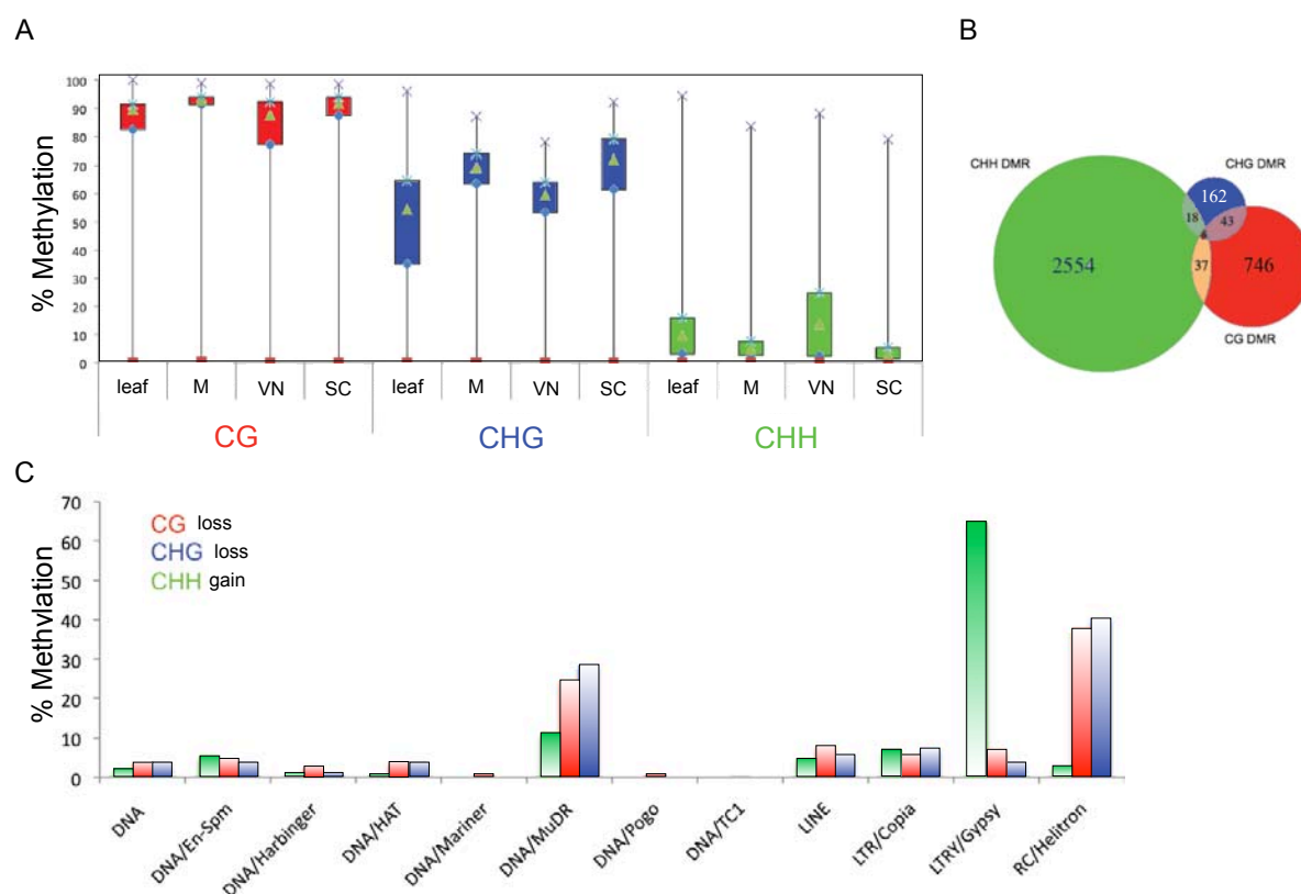
Figure 4.1 - Analysis of differentially methylated regions between microspores, sperm cells and vegetative nucleus. (A) Box plot representing DNA methylation percentages (minimum, lower quartile, median, upper quartile and maximum) at all TEs in the Arabidopsis thaliana genome. Overall, CG and CHG methylation is slightly lower in the VN compared to SC, microspore (M) and leaf, while CHH methylation is much higher in the VN compared to the SN. (B) Venn diagram showing that TEs with a statistically significant 3-fold change DMR between SN and VN do not overlap. TEs that lose CG or CHG methylation tend to have the same levels of CHH methylation. (C) Histogram showing the relative percentage of TE families that either lose CG/CHG or gain CHH in the VN. RC/Helitron and DNA/MuDR elements are the most represented TEs showing CG or CHG hypomethylation, while Gypsy, Copia and some MuDR and Helitrons show CHH hypermethylation.
