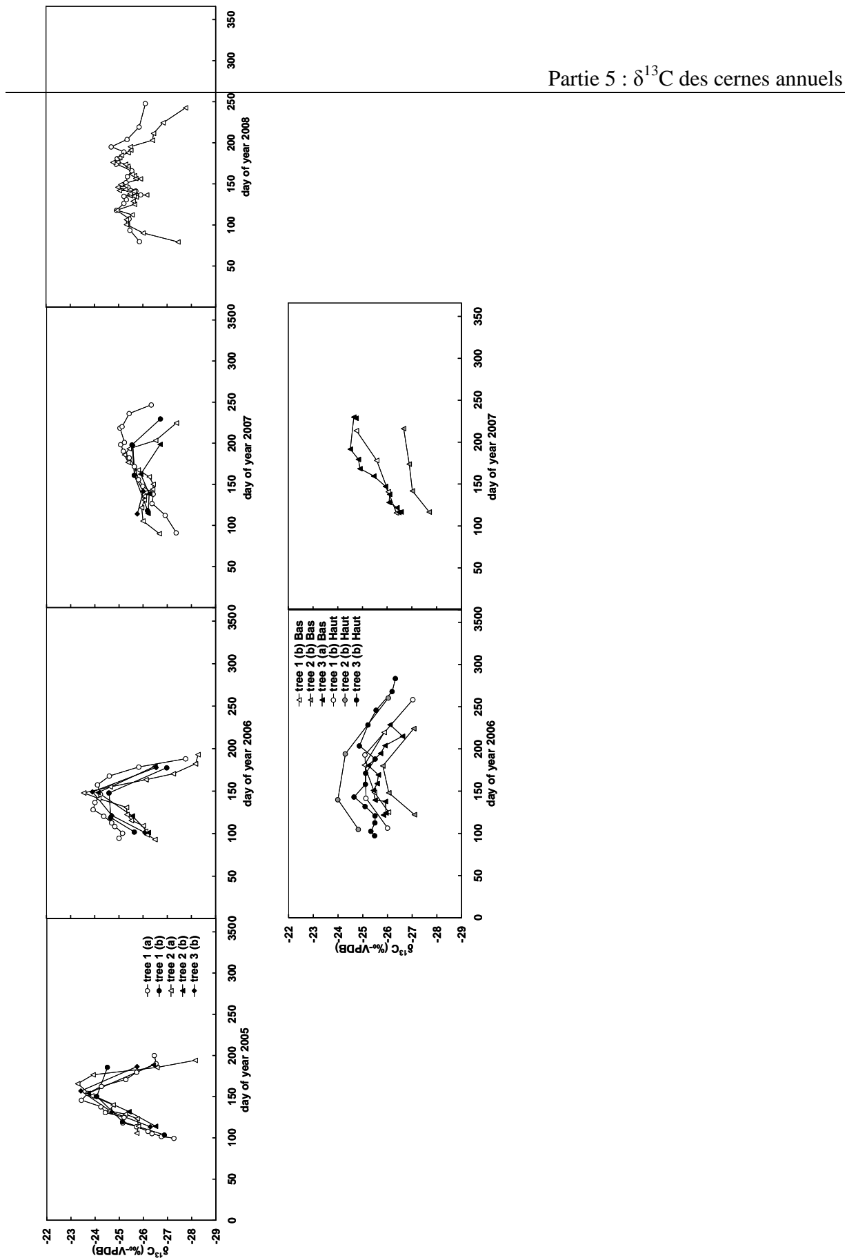
Figure 5. Intra-annual dynamics of the carbon isotope composition of cellulose synchronised with time using microdendrometric recordings and cellulose content of each ring fraction. Upper diagrams: trees from Le Bray site and years 2005 to 2008; lower diagrams: trees from Vielle Haut and Vielle Bas sites over the period 2006-2007.
