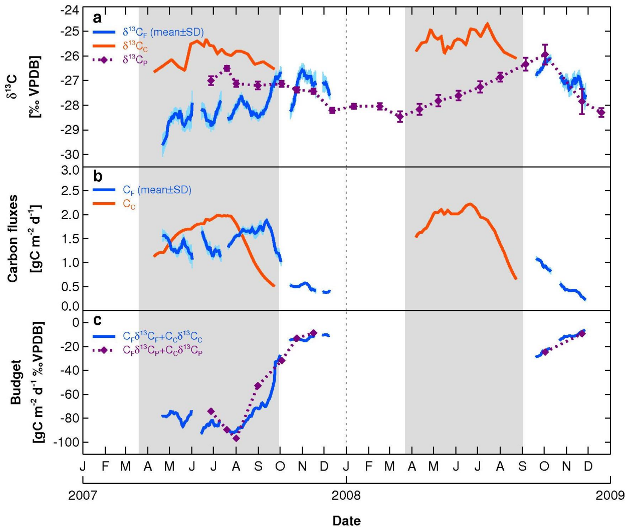
Figure 2 | Seasonal variations of (a) the carbon isotope compositions of wood cellulose ( \delta^{13}C_C ), phloem sugars ( \delta^{13}C_P ) and stem CO 2 efflux ( \delta^{13}C_F ), (b) the carbon fluxes allocated to stem respiration ( C_F ) and cellulose synthesis ( C_C ) and (c) the main two terms of the carbon budget at stem base. \delta^{13}C_P data consists of a mean value on 5 to 10 trees. Stem CO 2 flux data was collected at canopy height (16 m), while cellulose and phloem sampling was performed at stem base (1.3 m). In panels a and b, a 2-week flux-weighted moving average has been applied on the stem CO 2 efflux data. The shaded area indicates the stem growth period, estimated as the period when stem radial increment is above 0.0033 mm d -1 .
