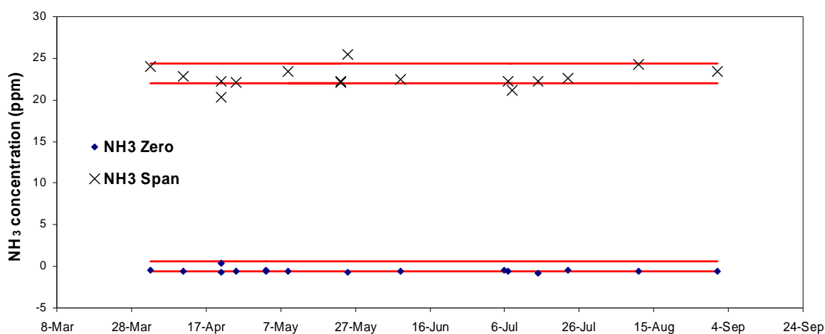
Figure 1. Behavior of the INNOVA 1412 when challenged and/or calibrated for NH 3 with zero (99.999% nitrogen) and span (23.2 ppm NH 3 balanced with nitrogen) during the course of some trials of the experiment. The lines represent a 0 \pm 0.5 ppm NH 3 tolerance range for the zero gas and 23.2 \pm 1.2 ppm NH 3 tolerance range for the span gas.
