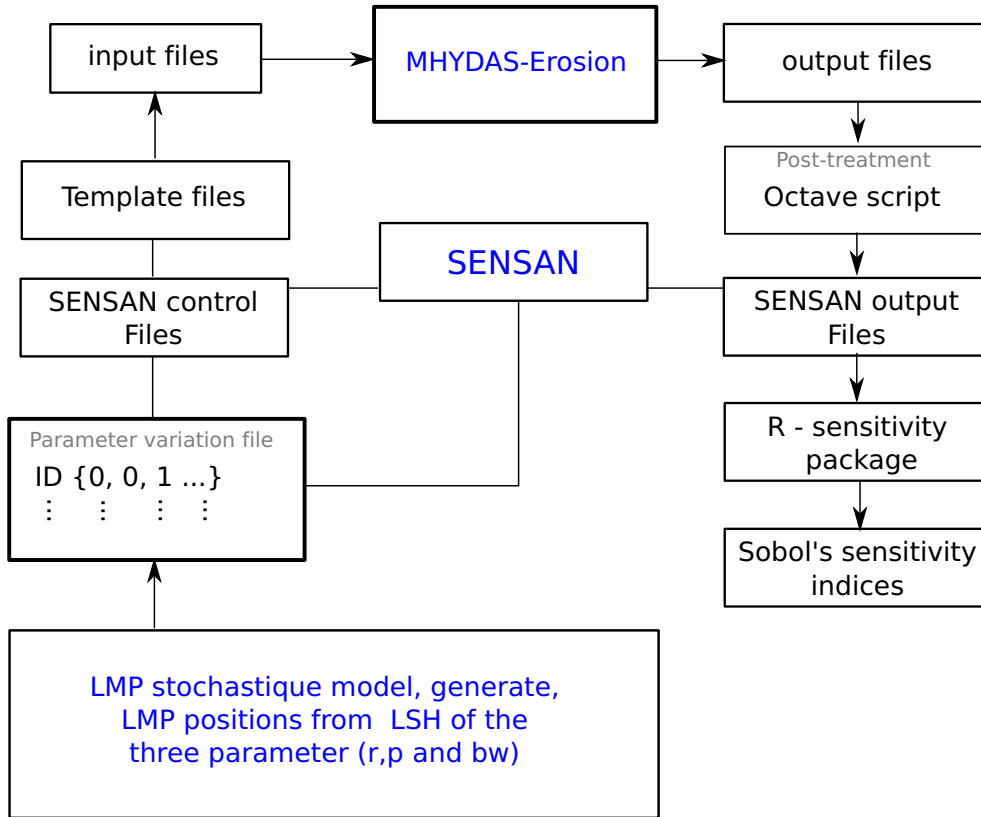
Figure 7.4: SENSAN scheme
