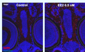
Fig 3: Microphotographs of 10 dpf zebrafish larvae control and exposed to EE2 - Effect on GnRH fibers immunoreactivity - Bar : 20 \mu m
