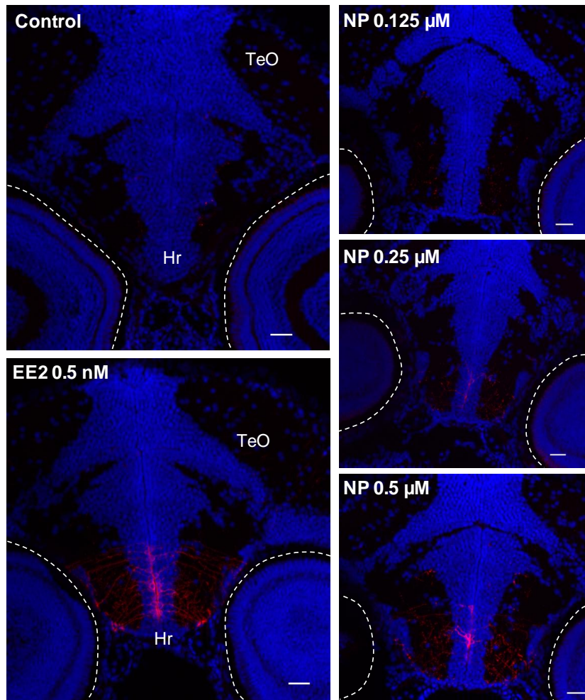
Figure 1 : AroB expression (red) in the brain of 7 dpf-old zebrafish from control and treated groups with either EE2 0.5 nM, NP 0.125 \mu\text{M} , NP 0.25 \mu\text{M} or NP 0. 5 \mu\text{M} . Microphotographs of transverse sections at the level of the rostral hypothalamus (200x magnification). TeO, tectum opticum; Hr, rostral hypothalamus. Dotted lines indicate eyes. Blue: Hoechst staining. Scale bars = 20 \mu\text{m} .
