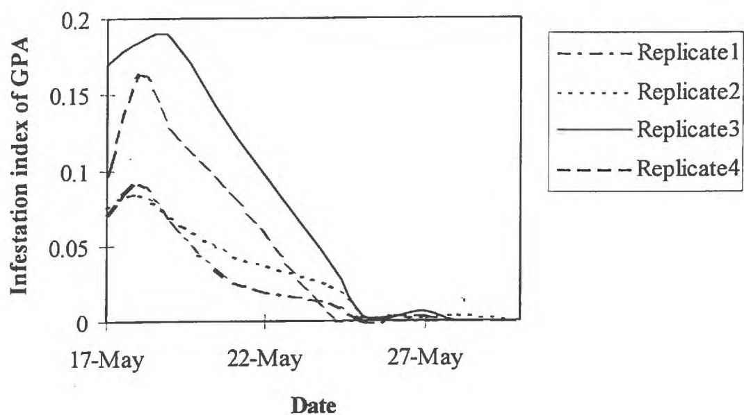
Fig. 6-2 Evolution of index of relative infestation of green peach aphids on encaged peach trees onto each of which 50 3 rd instar larvae of Harmonia axyridis were released on the 18 th of May.
