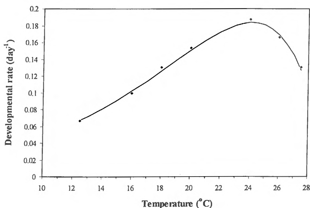
Fig. 2-1 Developmental rate D ( D=1 \text{ day}^{-1} ) of M. persicae in relation to constant temperature ( ^{\circ}\text{C} ). The curve is plotted using predicted values from equation (2-2); the dots are observed values.
