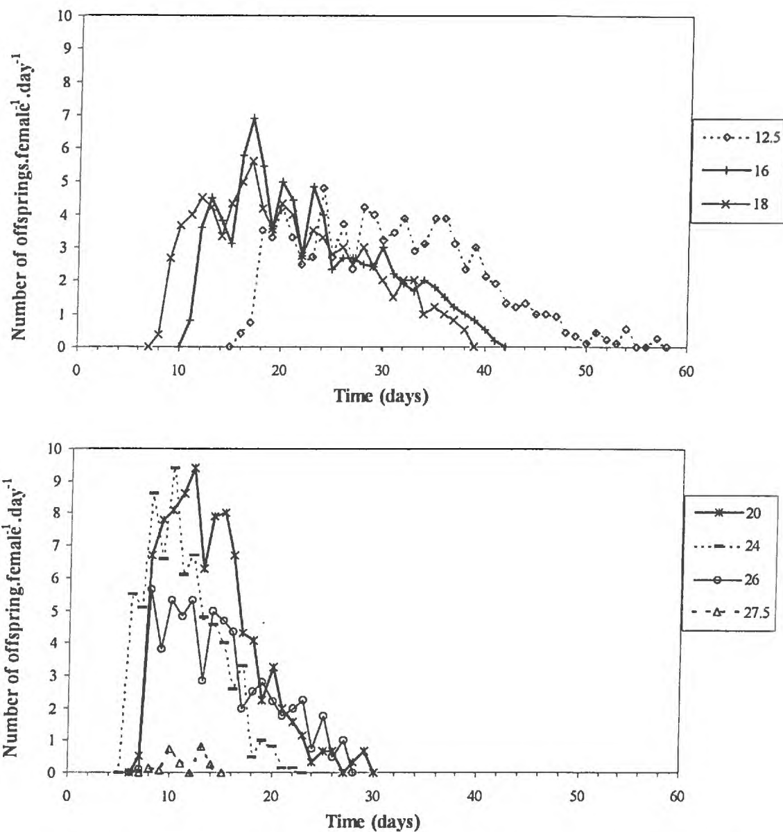
Fig. 2-3 Age-specific fecundity profiles of M. persicae in relation to temperature (°C). Observation made under laboratory conditions. The aphids are reared on peach seedlings cultivated in nutritive solutions. Photoperiod is set at 14:10. The numbers in the legend boxes are temperatures in °C
