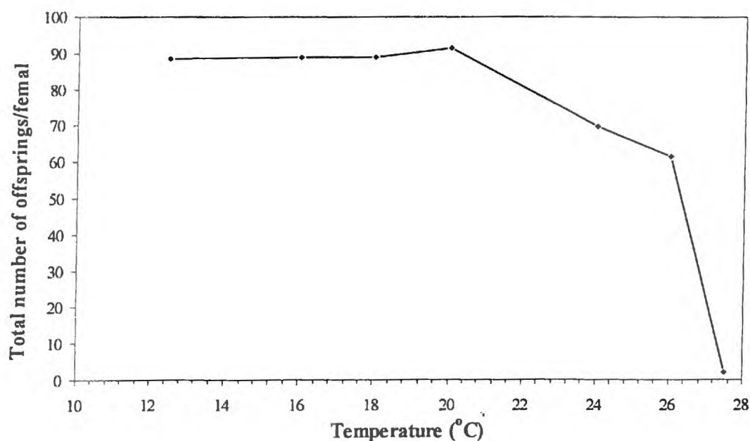
Fig. 2-2 Relationship between the total fecundity of M. persicae and temperature (°C) on peach seedlings cultivated with nutritive solution under laboratory conditions. Photo period 14:10.
