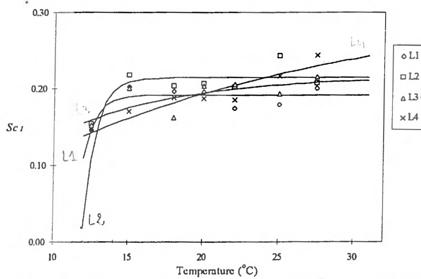
Fig. 4-6 Relationship between the parameter Sc_1 from Eqn. 4-3 and temperature ( ^{\circ}\text{C} ). Solid lines are drawn using predicted values from Eqn. 4-8, marks are observed values.
