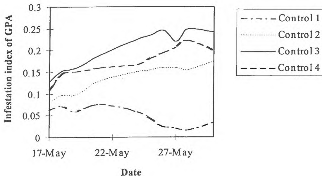
Fig. 6-1 Evolution of index of relative infestation of green peach aphids on encaged peach trees with larvae of Harmonia axyridis .
