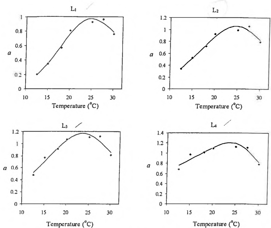
Fig. 3-2 The relationship between instantaneous attack rate a of H. axyridis on M. persicae and Temperature ( ^{\circ}\text{C} ). L1-4 denotes the larval stadium 1-4.
