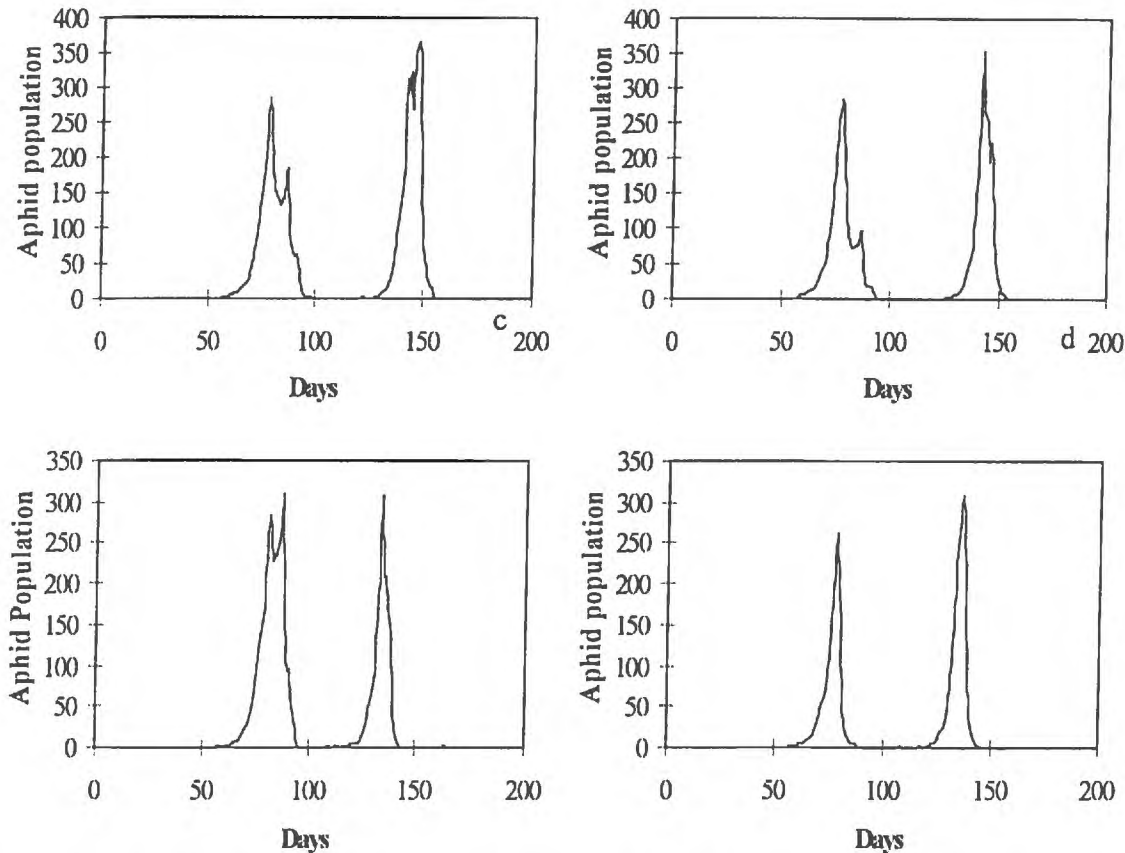
Fig.5-10. Simulated population change of green peach aphid under varying temperature when increasing the number of larvae of Harmonia axyridis for the first release at the aphid population density of 250/colony. The Instar and quantity of larvae of Harmonia axyridis released --- a: 1 st instar 5-1; b: 2 nd instar 4-1, c: 3 rd instar 3-1, d: 4 th instar 3-1. Temperature data are generated using CLIMGEN, a climate data generator developed by USDA-ARS, with parameters calculated from the local meteo record maintained by INRA-Station de Agroclimatologie at Montfavet.
