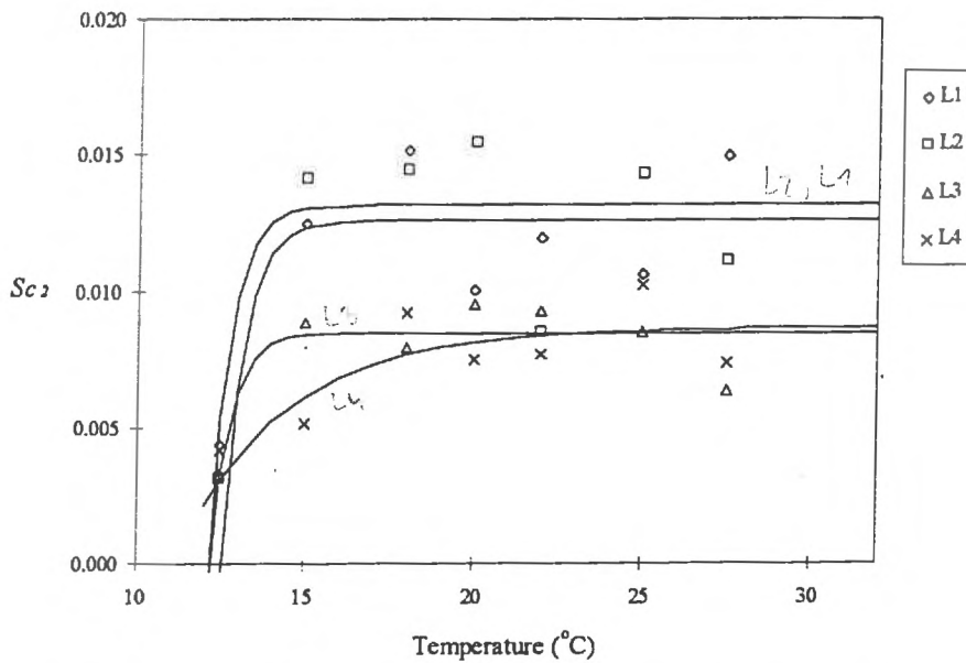
Fig. 4-7 Relationship between the parameter Sc_2 from Eqn. 4-3 and temperature ( ^{\circ}\text{C} ). Solid lines are drawn using predicted values from Eqn. 4-9, marks are observed values.
