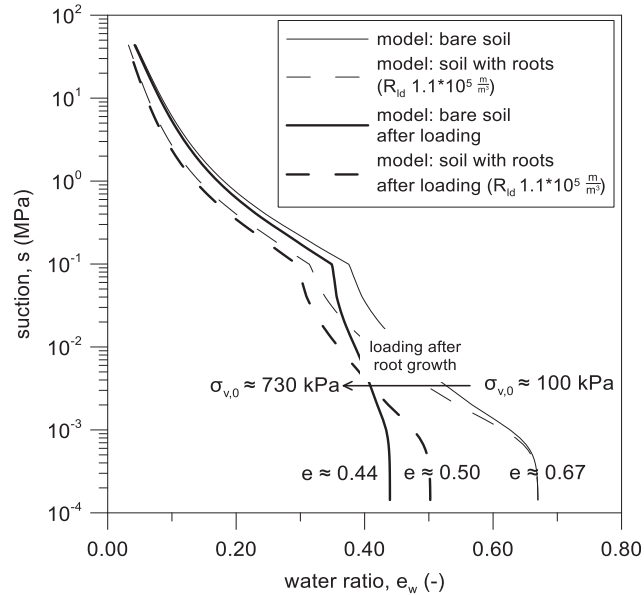
Figure 27 Prediction of bare and vegetated swrc before and after loading.
