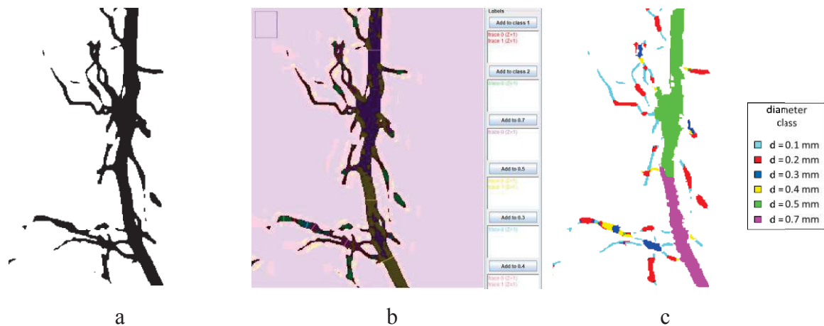
Figure 35 Image treatment to calculate the average root length for each diameter class. A) original binarized image, b) machine training with recognised diameters Sections (lines), c) roots characterized by diameter's classes.
