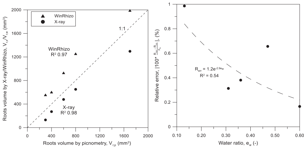
Figure 6 Comparison of values of roots volume obtained from the different techniques and b) potential relative error in porosity between measurements done with X-ray micro-tomography and pycnometry.
