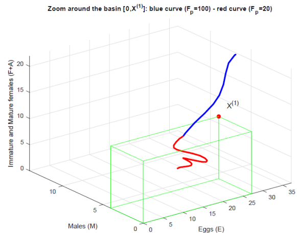
Figure 3.10: Control with first F_p = 100 , then F_p = 20 once the system has reach the basin of attraction of \mathbf{0} (dotted lines) for a control starting at t_{start} = 390 : (a) trajectories of the system (b) Zoom of the trajectory near [0, X^{(1)}] .
