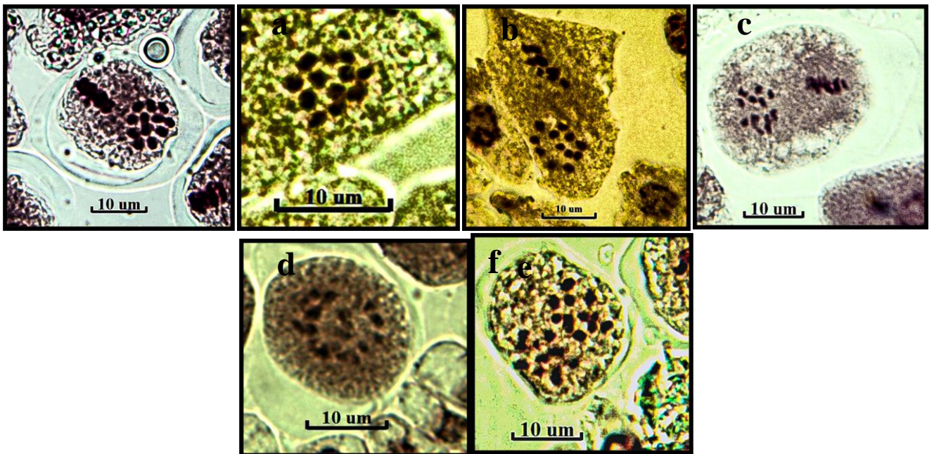
Fig. 1: Meiotic plates of the studied species. (Les lettres a, b c....etc à mettre en blanc sur la figure)
