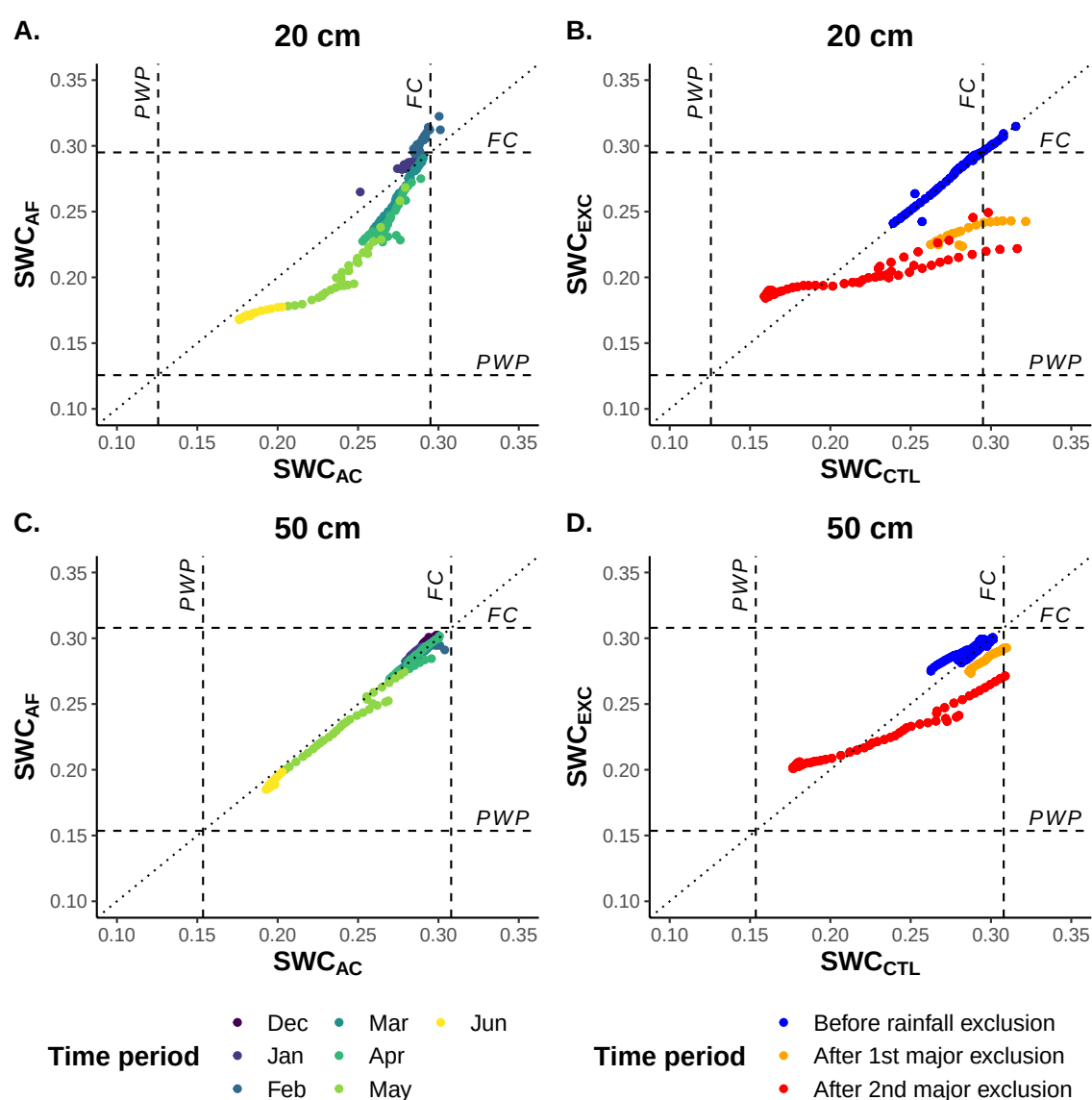
Figure II.4 Paired analysis of mean daily soil water content (SWC) [ m^3.m^{-3} ] between cropping systems (A. and C.) and rainfall regime (B. and D.) at 20 and 50 cm depth. Dotted line indicates 1:1 line and dashed lines indicate permanent wilting point (PWP) and field capacity (FC) computed according to Rawls et al. (2003). Colors indicate different time period, set as i) 1-month interval for the evaluation of SWC dynamics between cropping systems and as ii) interperiod between major rainfall exclusion ( > 20 mm) for the evaluation of dynamics between rainfall regime.
