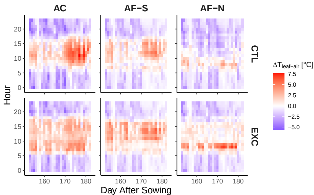
FIGURE E.9 Difference between leaf and air temperatures from mid-flowering until seed maturation, in different cropping systems and rainfall regimes.
