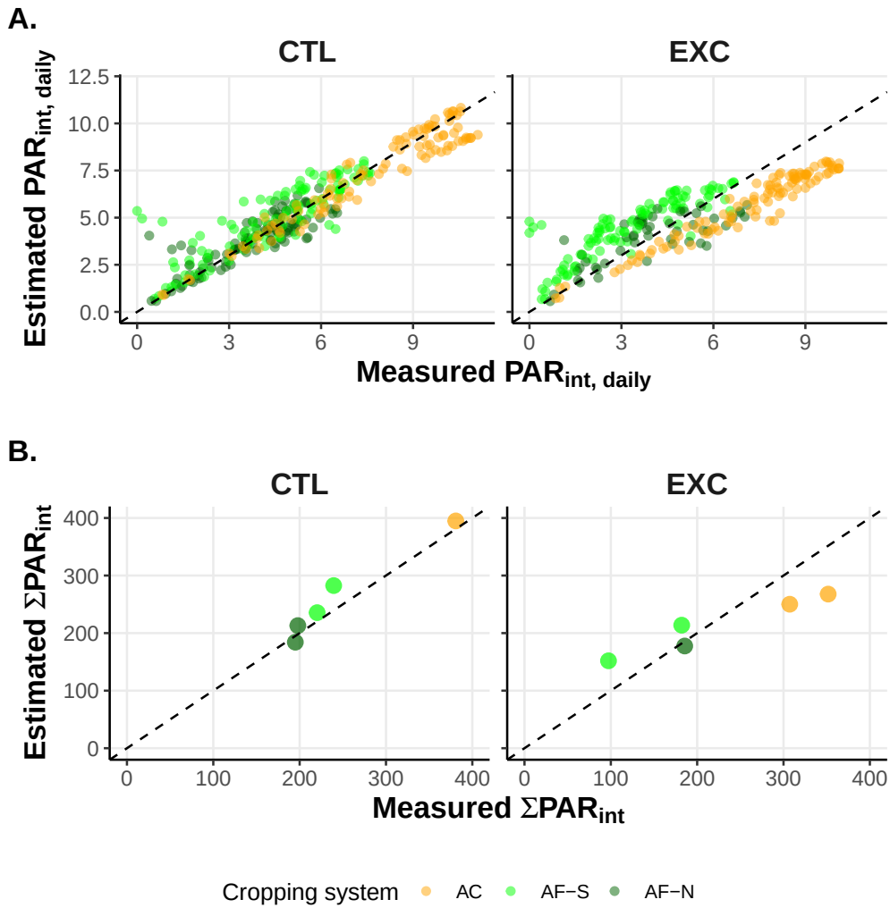
FIGURE E.4 Comparison of daily intercepted PAR ( PAR_{int} ) measured with PAR sensors and calculated from the LAI value using the Beer's law in all cropping conditions. Dashed line represents 1 : 1 line.
