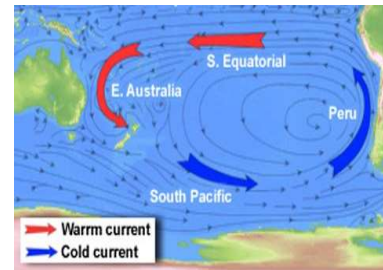
Figure 5 : Principaux courants marins dans le Pacifique. COMET® Website at http://meted.ucar.edu/ of the University Corporation for Atmospheric Research (UCAR).
