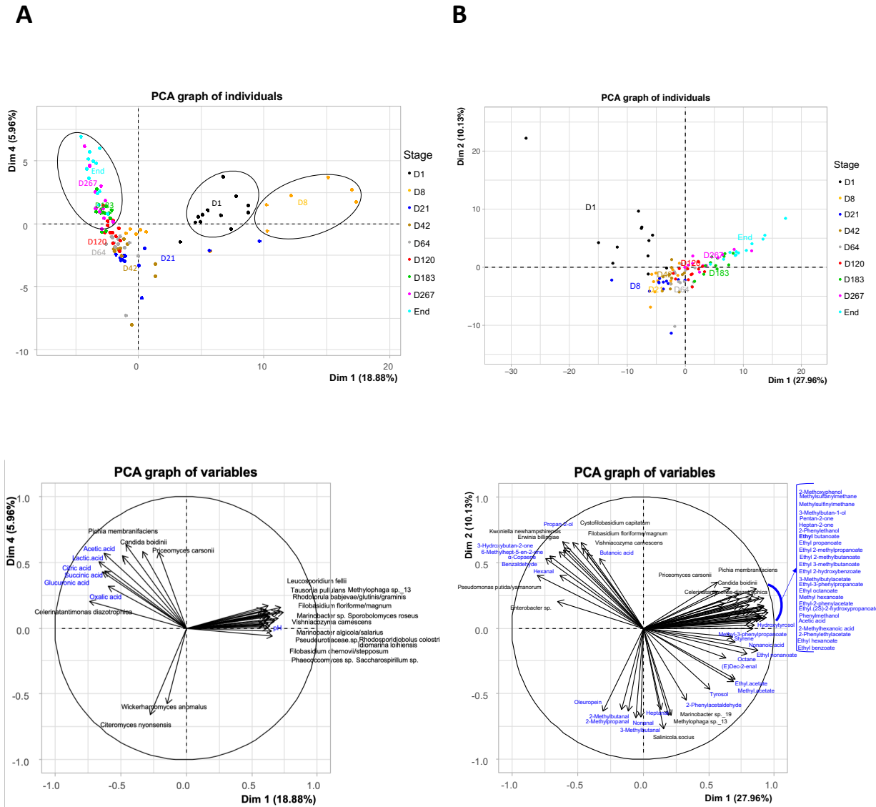
Supplementary Figure S7. Principal component analyses of microbial culture-independent and biochemical data (acids and volatile compounds in blue) throughout fermentation in brine (A) and in olive fruit (B). For both matrices, individual and variable plots are presented with sampling times considered as individuals. Variable plots considered species abundances (black) and organics acid concentration for brine and volatile compounds for olive fruit (blue).
