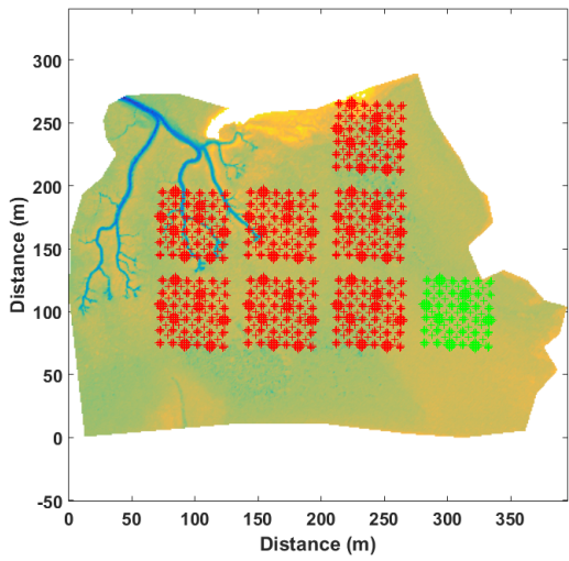
Appendix L3: As Appendix L1 but for Gibraltar Point (natural saltmarsh)
