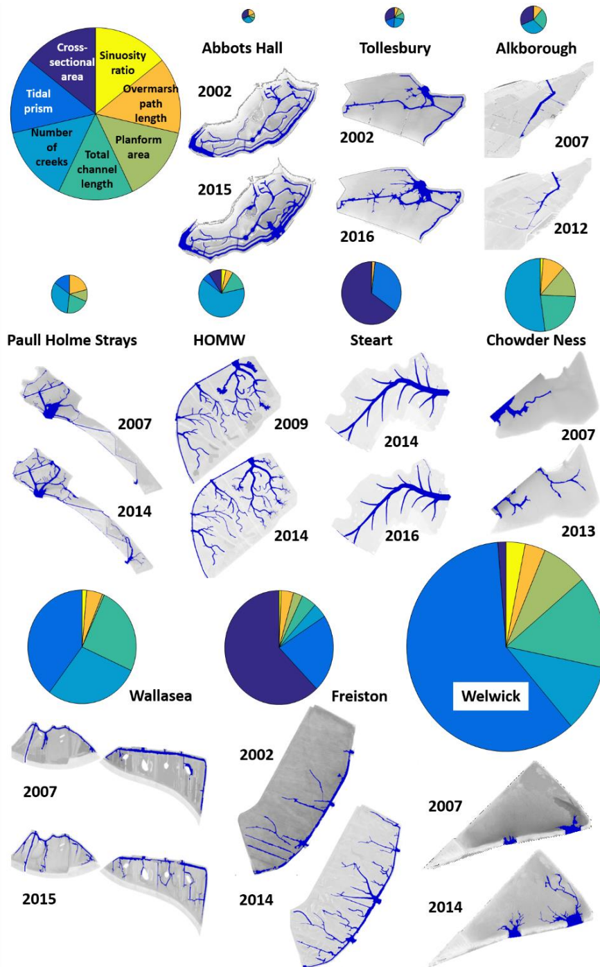
Figure 7.16: MR schemes ranked by total normalised evolution rates (creek extent for the first and last year of monitoring shown in blue). The evolution rates pie plots are invisible at this scale for the 2 AR sites, indicating a negligible evolution compared to the younger breached sites.
