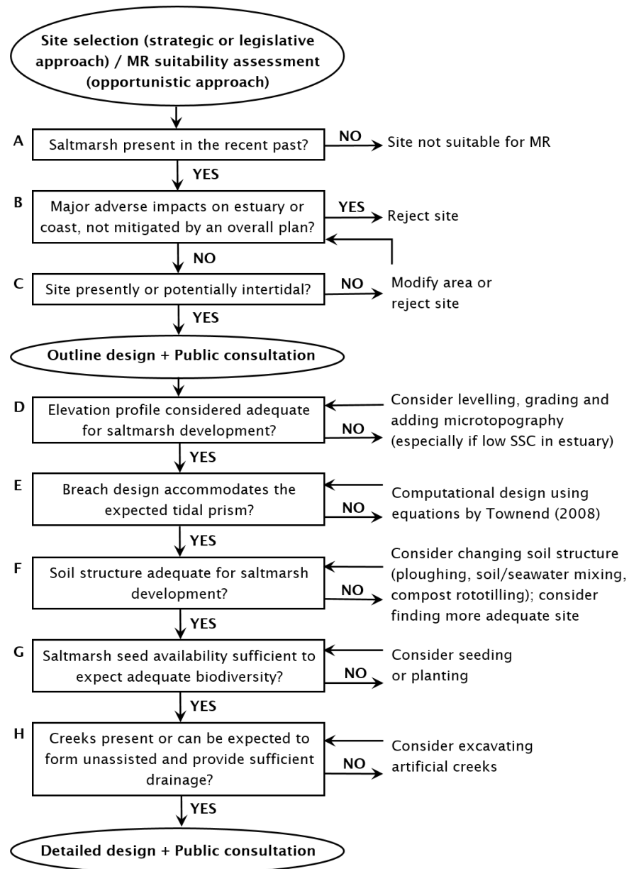
Figure 2.8: Ecomorphological planning and design of MR, not taking into account socioeconomic considerations. A-C: considerations for MR site selection or suitability assessment; D-H: considerations for MR design. SSC= Suspended Sediment Concentration. Compiled based on information from Burd (1995); Leggett et al. (2004); Nottage et al. (2005); O'Brien et al. (2006); Mossman et al. (2012); Brooks et al. (2015)
