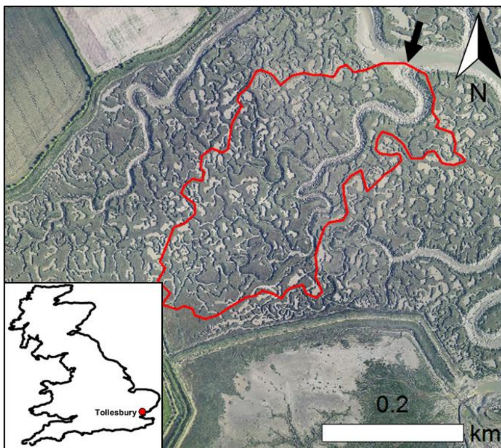
Figure 3.6: Aerial photography of Tollesbury (20 cm resolution composite image from three flights on the 15/07/2011, 15/08/2011 and 14/09/2011, Environment Agency). Outlet shown by black arrow. MR extent considered shown by red line.
