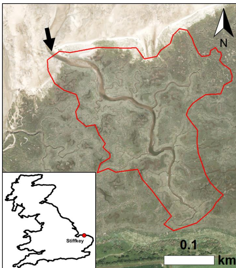
Figure 3.10: Aerial photography of Stiffkey (20 cm resolution composite image from two flights on the 12/06/2014 and 31/10/2014, Environment Agency). Outlet shown by black arrow. MR extent considered shown by red line.
