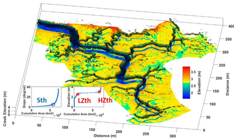
Figure 4.2: Creek elevation and slope threshold detection at Stiffkey Marsh (step 1). Sth: blue circle. HZth, LZth: red asterisks. The logical mask detected with those thresholds is displayed in black over the lidar elevation map.
