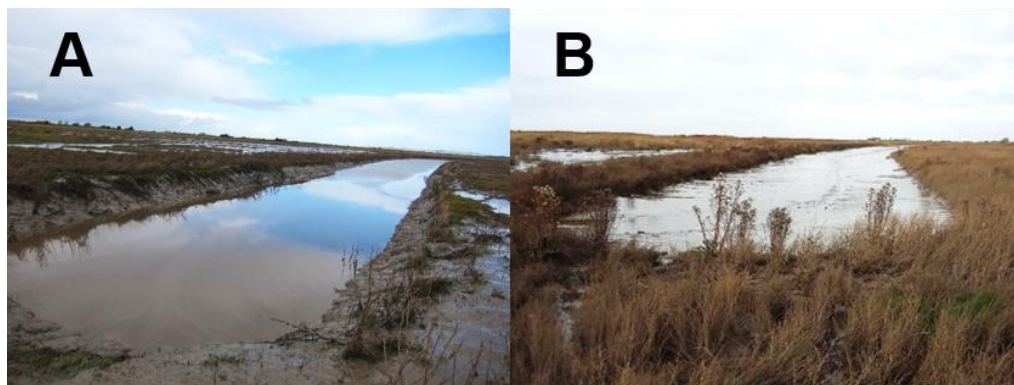
Figure 8.1: Infill of large creek at Steart between 23/02/2015 (A: photo taken by Anas Annuar) and 16/11/2016 (B: photo taken by Matthey Agius)
