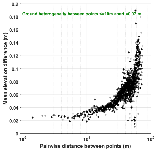
Appendix L3: As Appendix L1 but for Gibraltar Point (natural saltmarsh)
