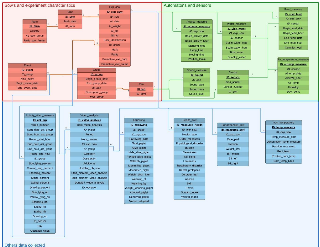
Figure 3-1: Schema of the relational database.
