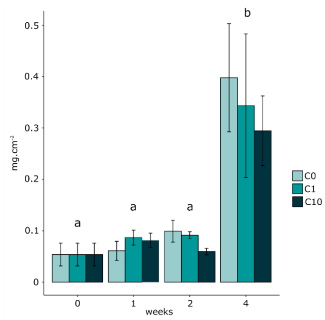
Figure 3.1. Biofilm biomasses over time in control (C0 = 0.2 \pm 0.1 nM) and Zr exposures (C1 = 0.5 \pm 0.3 nM and C10 = 2.9 \pm 0.3 nM). Values are averages and standard errors. Two-way ANOVA was performed to detect significant differences between exposure times, and these differences are indicated by letters ( p < 0.05 ; n = 3 ).
