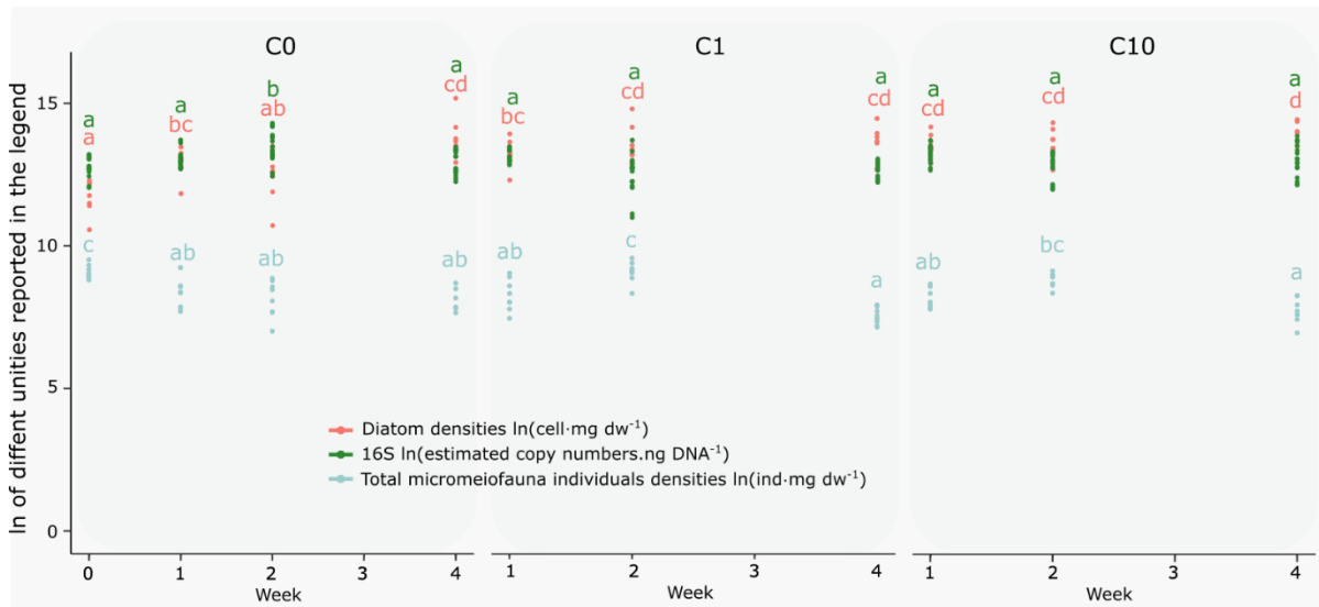
Figure 4.1. Total individuals (ln) normalized by biomass (live diatoms per mg of dry weight in red, number of Eubacteria 16s ARN genes copies obtained by qPCR per ng of total DNA sample in green, micrometazoans individuals per mg of dry weight in blue) observed over time in control C0 ( 0.004 \pm 0.002 nM Th) and Th exposures (C1 = 0.18 \pm 0.09 nM Th and C10 = 8.7 \pm 3.4 nM Th). A two-way ANOVA was performed to detect significant differences between treatments, indicated by letters ( p < 0.05 ; n = 8 ).
